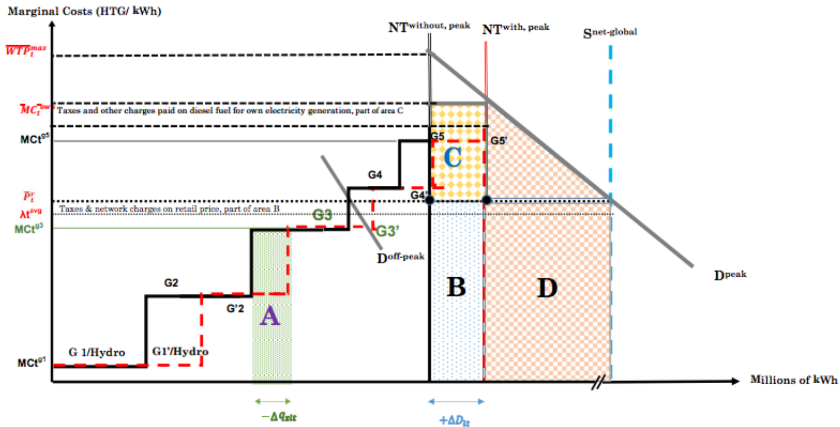
Figure 8. Economic Analysis of an Improved Transmission Line Efficiency
