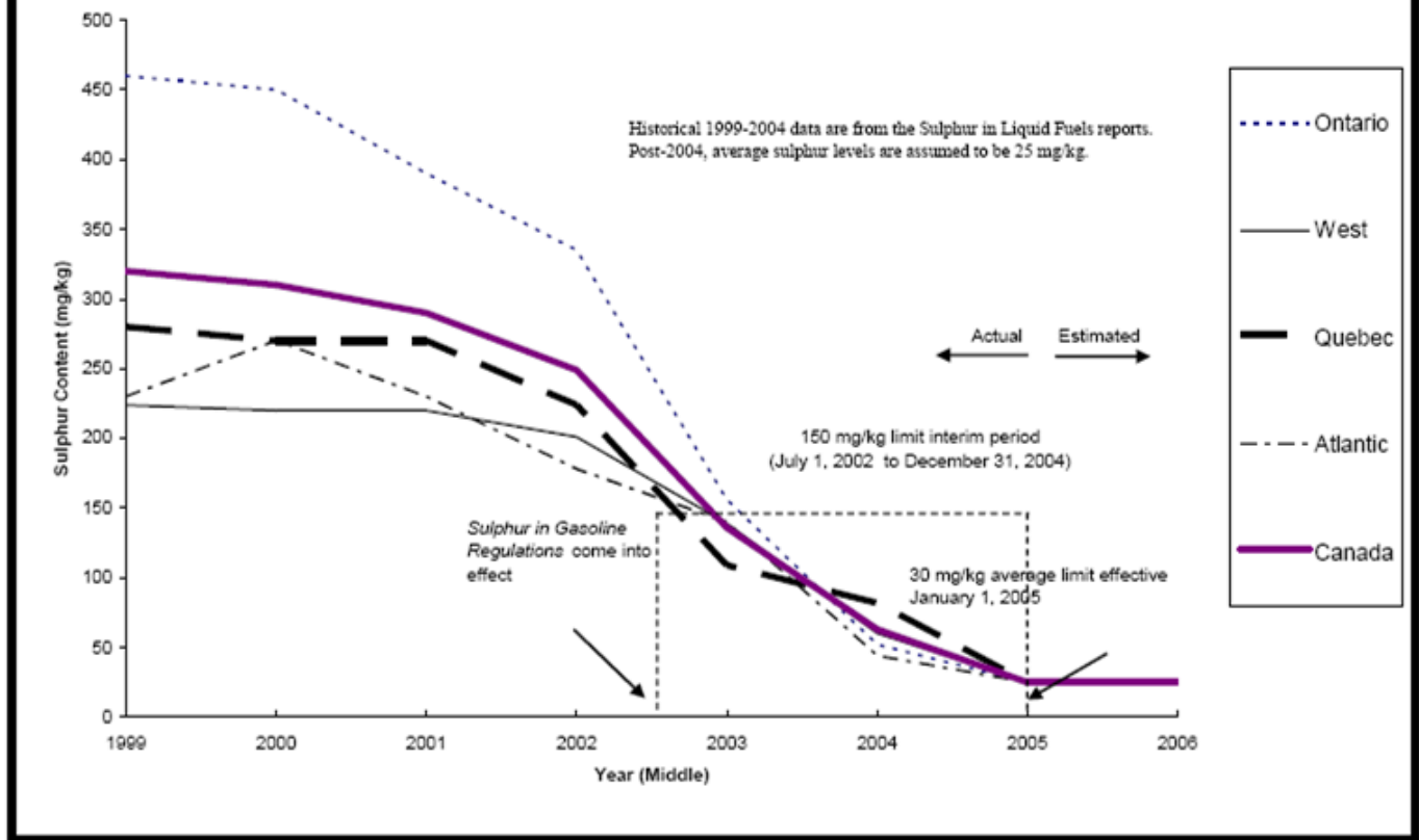
Figure 1: National Trend of Sulphur Content in Gasoline (1999-2006)
